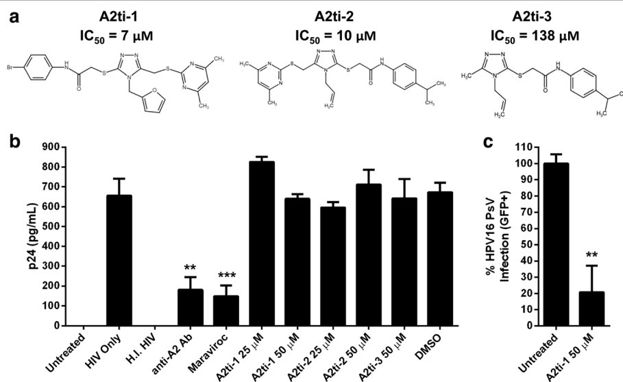
Fig. 2 in vitro HIV-1 infection of macrophages following treatment with A2ti, anti-A2 antibody, or maraviroc. a Structures and reported IC 50 values of the three triazole-based A2ti tested [13]. b Macrophages were treated with different A2ti (25 or 50 µM), an anti-A2 antibody (25 µg/mL), or maraviroc (25 µg/mL) prior to exposure to HIV-1 JR-CSF (MOI = 1). After 24 h, the supernatants were collected and the relative amount of the HIV-1 capsid protein p24 (pg/mL) was measured via ELISA. Controls included uninfected, HIV only, heat-inactivated virus (H.I. HIV), and DMSO at a concentration matched to that of 50 µM A2ti. Data are presented as the means ± SD of three independent experiments. ** p < 0.01 and *** p < 0.001 as determined by unpaired two-tailed Student's t -tests compared to the HIV only group. c HaCaT cells were left untreated or treated with 50 µM A2ti-1. The following day cells were infected with GFP-plasmid-containing HPV16 pseudovirions (Psv). GFP-positive cells were measured after 48 h by flow cytometry. The mean percentage ± SD of infected cells normalized to the untreated group from a representative experiment performed in triplicate is presented. ** p < 0.01 as determined by unpaired two-tailed Student's t -test compared to the untreated group
