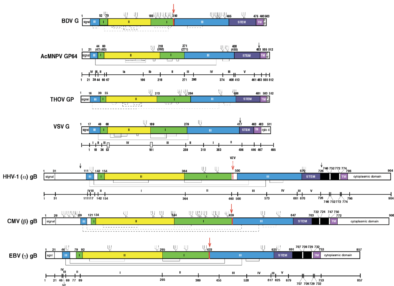
Figure 2 Similar linear arrangement of putative domain structures of BDV G, VSV G, THOV GP and AcMNPV GP64 and herpesvirus gB. Class III VFP domain nomenclature and coloring is as in Fig. 1. Amino acids are numbered beginning after the putative signal sequences in VSV G, but at the beginning of the signal sequence of HSV-I gB. Arrows indicate G and gB truncations of the forms used for crystallography. Solid lines represent cysteine bonding in VSV G, AcMNPV GP64, and HSV-I and EBV gB [30,32,34,43]. Black boxes represent hydrophobic regions, with violet representing the transmembrane anchor (TM). Dashed lines represent potential cysteine bonding in BDV G, THOV GP and CMV gB. Dashed arrow is the location of a furin cleavage site in the alpha herpesvirus varicella zoster virus (human herpes virus 3). Solid arrows are furin cleavage sites in BDV G, CMV gB, and EBV gB.
